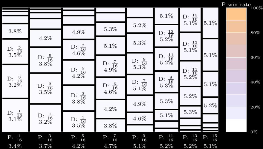
Plaintiff Signals
